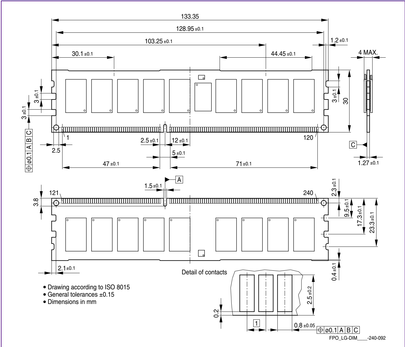
FIGURE 3 Package Outline LG-DIM-240-092 R/C B
