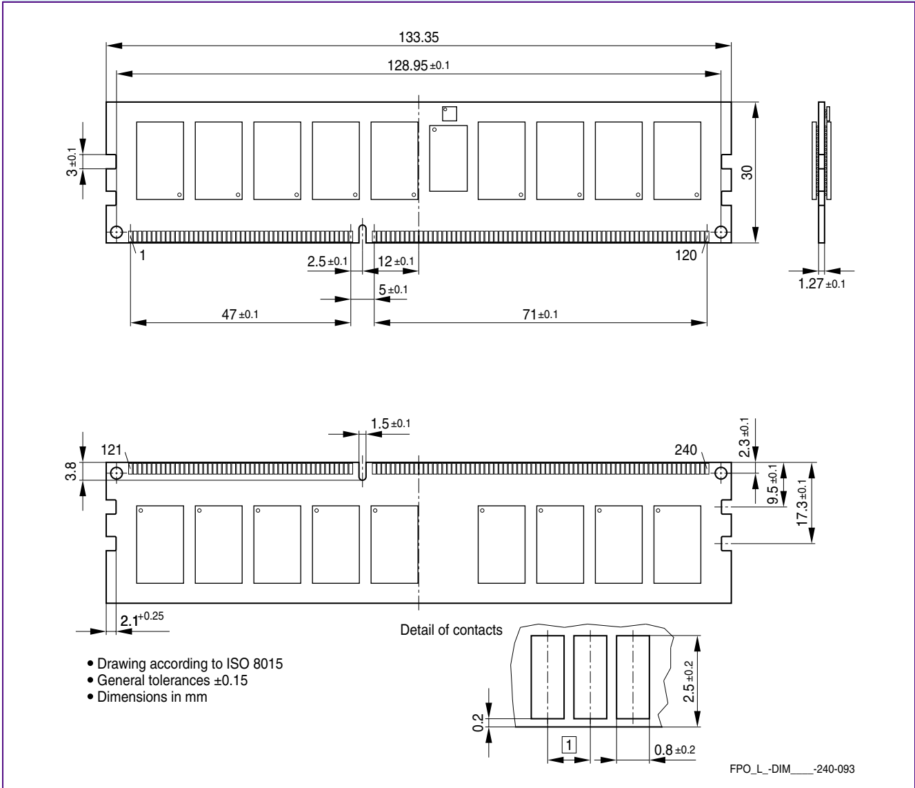
FIGURE 4 Package Outline LG-DIM-240-093 R/C C
