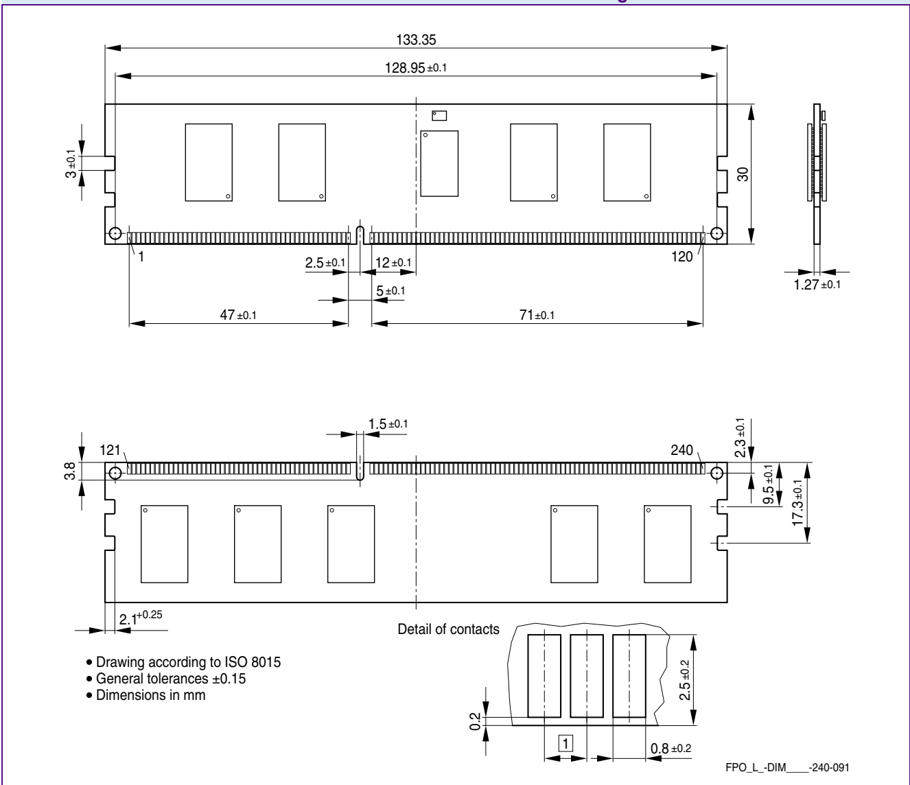
FIGURE 2 Package Outline LG-DIM-240-091 R/C A
