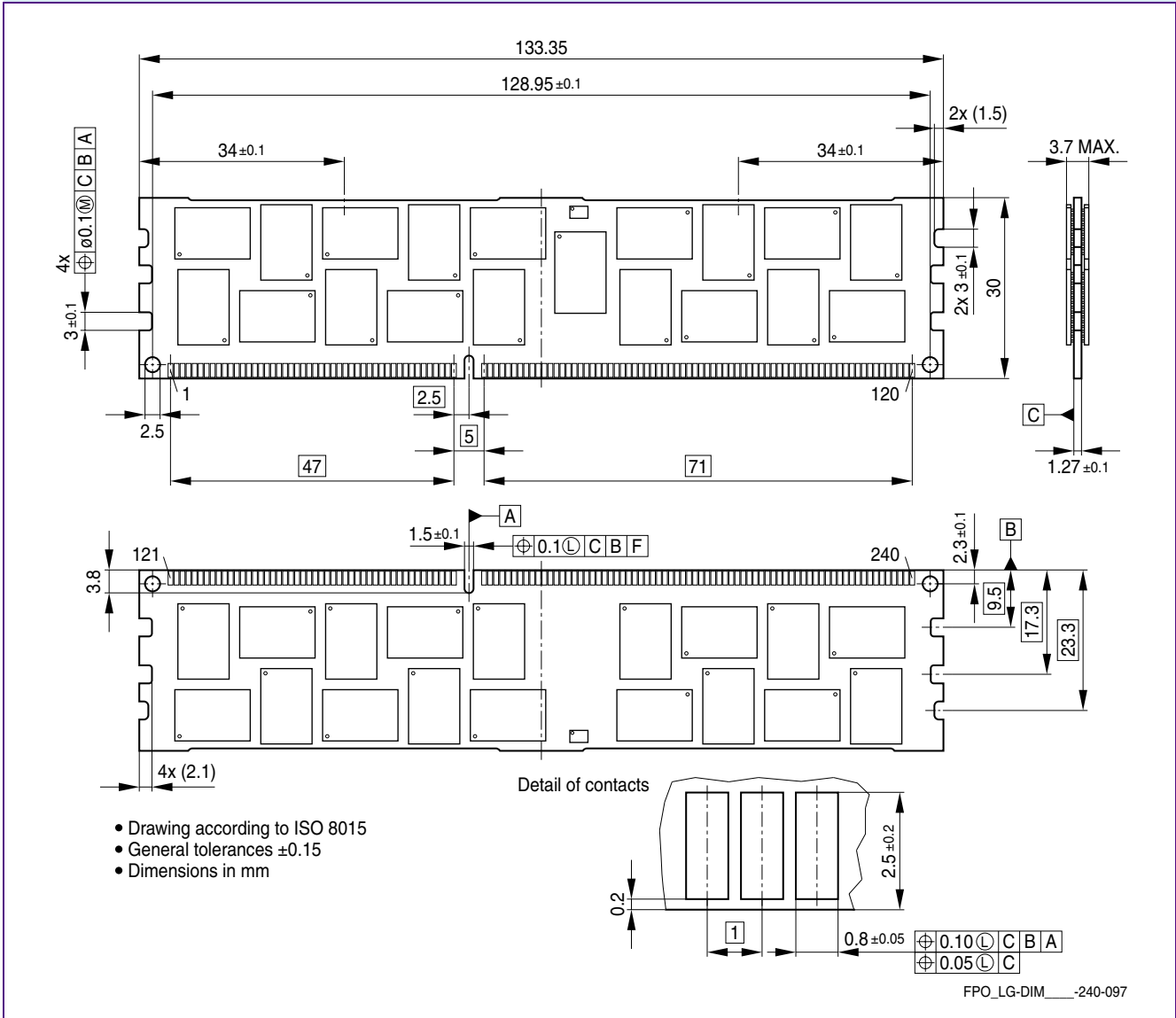
FIGURE 5 Package Outline LG-DIM-240-097 R/C E
